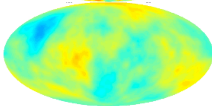
ISW ( z < 3 )
