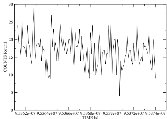
Fig. 2.— Lightcurve for pn with 100 s binning.
