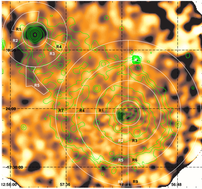
Fig. 12.— Hardness ratio map of A1644, based on the ratio of the combined MOS1-MOS2-pn count rates in the energy bands 0.3–2.0 keV and 2.0–10.0 keV. The map has been corrected for background, exposure, and vignetting, and is adaptively smoothed. Soft emission appears dark and hard emission bright. Also shown are surface brightness contours from Fig. 5 and regions selected for spectral analysis.
