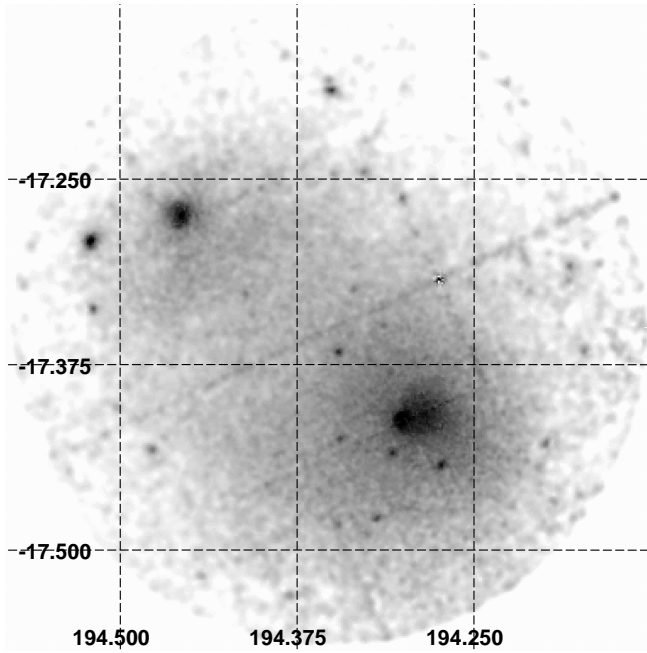
Fig. 4.— Background, exposure, and vignetting corrected, adaptively smoothed, combined MOS1-MOS2-pn count rate image of A1644 in the energy range 0.3–5.0 keV (R.A. and Dec. in equatorial coordinates, epoch J2000.0). The linear artifacts are due to an imperfect exposure correction near the chip boundaries.
