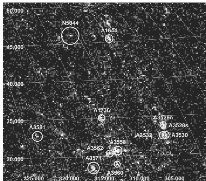
Fig. 1.— Location of A1644 relative to the core of the Shapley supercluster in Galactic coordinates. Shown are virial radii of a few clusters from Reiprich & Böhringer (2002) on top of a distribution of 2MASS galaxies.
