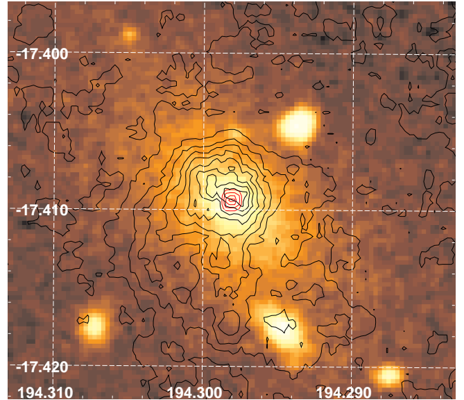
Fig. 6.— The DSS image of the inner region of the main clump, overlaid with the X-ray contours from Chandra (black) and, in the very center, the 1.4 GHz radio data (red; from M. Ledlow).
