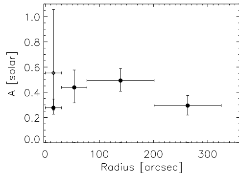
Fig. 11.— Metal abundance profiles for the sub clump. The open diamond shows the best fit abundance if a third thermal component is included.
