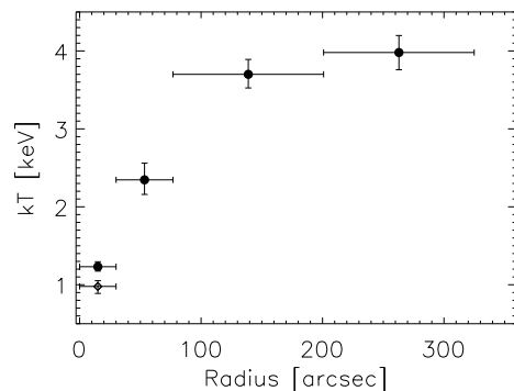
Fig. 9.— Radial temperature profile for the sub clump. The open diamond shows the best fit temperature if a third thermal component is included.
