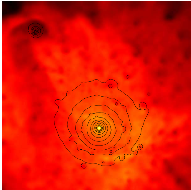
Fig. 18.— Mass weighted temperature map from a hydrodynamical simulation. Temperature increases from black to red to yellow. Also shown are X-ray surface brightness contours.
